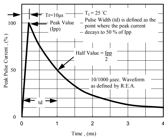
Fig. 5 - Pulse Waveform
